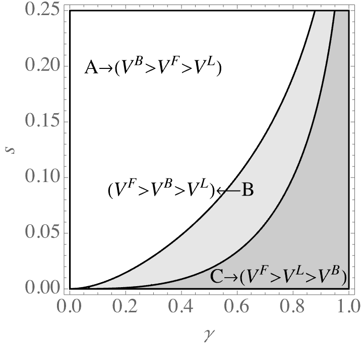
Figure 1: Total value rankings with region A: V^B > V^F > V^L ; region B: V^F > V^B > V^L ; and region C: V^F > V^L > V^B .
