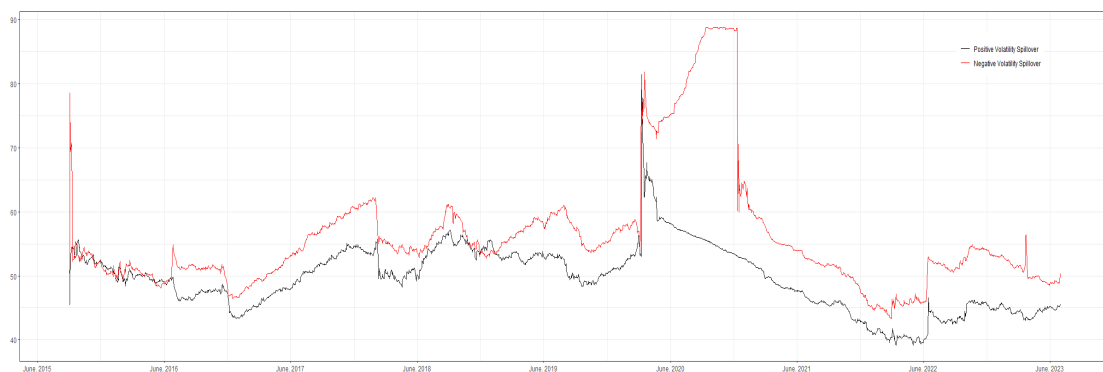
Fig.10: Dynamic total volatility spillover
