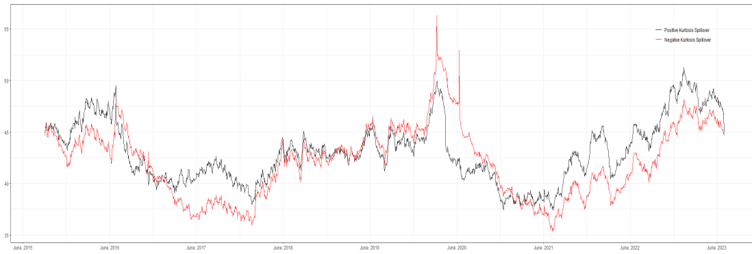
Fig.11: Dynamic total kurtosis spillover
