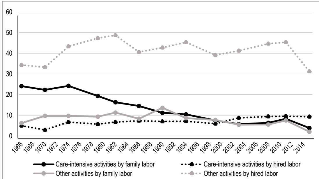
Figure 5. Changes in family and hired labor use (person-days/ha) for care-intensive and other activities during the wet season in Central Luzon, 1966–2015
