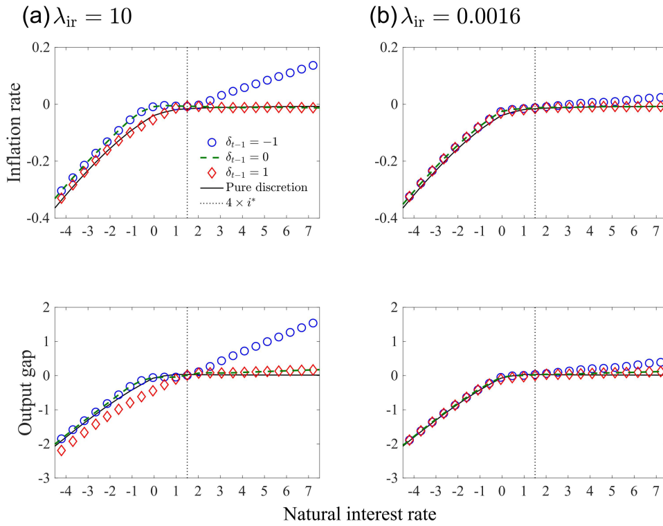
Figure S2: Policy functions for inflation and output gap. Black solid line denotes a pure discretionary policy without reversal aversion (i.e., \lambda_{ir} = 0 ). Blue circle, green dashed and red diamond respectively denote irreversible policies when the sign of policy shift in the previous period is -1 , 0 and 1 . We set i_{t-1} = i^* = 1.5/4 (vertical dotted line).
